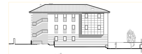
ALZADO PRINCIPAL
